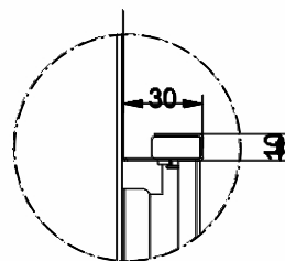
DETAIL A 1:2
