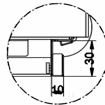
DETAIL A 1:2
