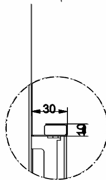
DETAIL A 1:2
