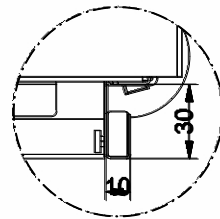
DETAIL A 1:2
